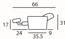
Recliner Mechanism
