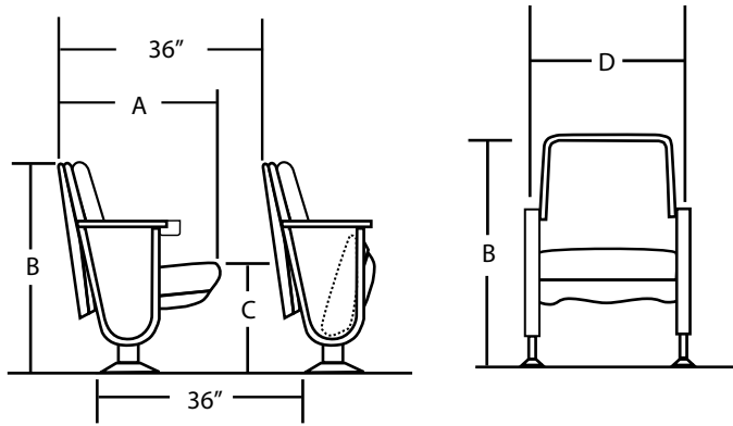
ROCKERS SEATING DIMENSION CHARTS
