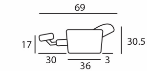
WALLSAVER Recliner Mechanism
