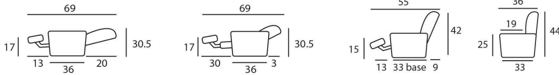
STANDARD Recliner Mechanism
