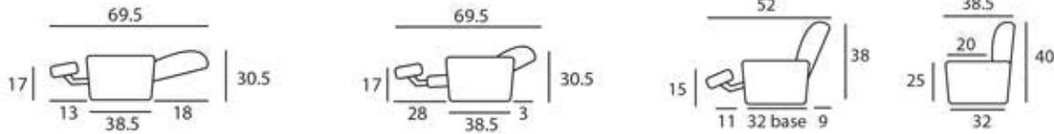
STANDARD Recliner Mechanism
