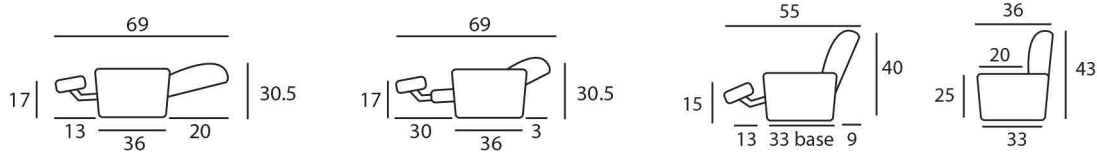
STANDARD Recliner Mechanism
