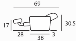
WALLSAVER Recliner Mechanism
